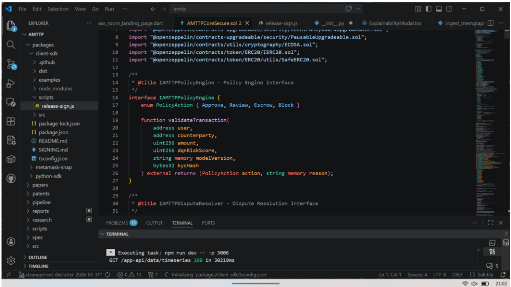
Figure 1: VS Code showing the core AMTTPCoreSecure.sol contract — the IAMTTPPolicyEngine interface that defines the four compliance outcomes (Approve, Review, Escrow, Block) and the validateTransaction function signature. The live War Room terminal (port 3006) confirms active development of the product layer alongside the contract layer.
