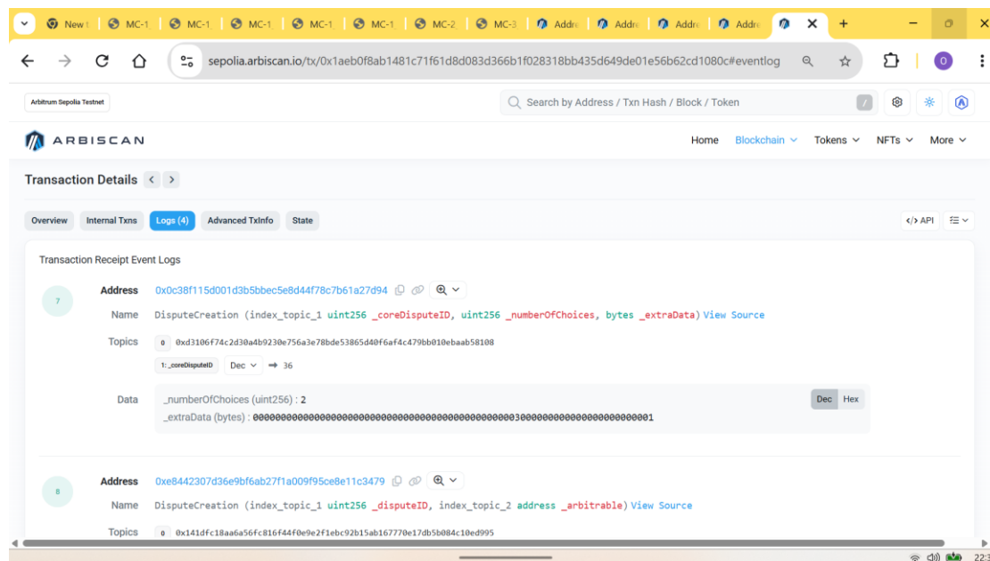
Figure 4: Arbiscan.io — DisputeCreation event on real Kleros v2 KlerosCore (Arbitrum Sepolia, chain 421614). AMTTPDisputeResolver 0x3A3b4F5aBa950c56bfc4a654fBAe873D2F91ed25 is registered as IArbitrable party in dispute #36, confirming the Kleros integration is live on the public testnet.
